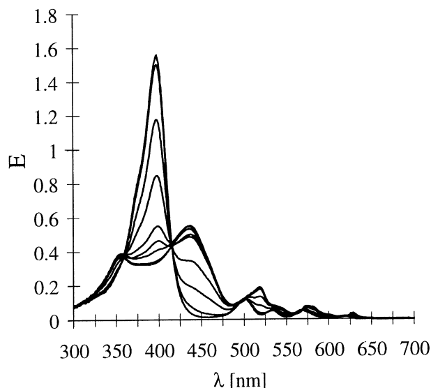
Figure 3. Optical spectra of 12 in methanol/water mixtures. Two isosbestic points were detected at 355 and 413 nm.
