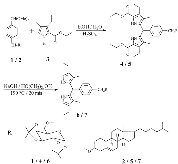
Scheme 1. Synthesis of dipyrlylmethanes.
