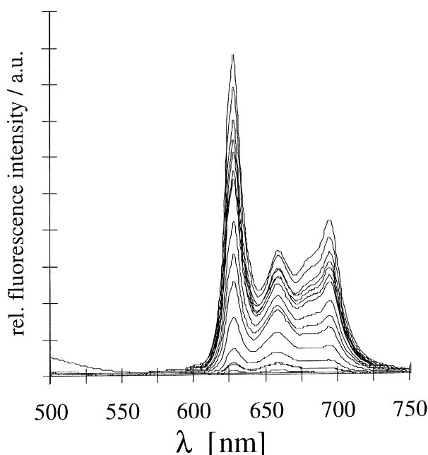
Figure 4. Fluorescence spectra of 12 in PE liposomes. The liposome concentration was varied from 5 (lowest curve) to 300 \mu\text{g/mL} (upper curve). Porphyrin concentration 2.5 \mu\text{g/mL} . Emissions at 625 and 688 are due to porphyrin monomer fluorescence, emission at 660 nm is due to fluorescence of porphyrin dimers incorporated in the liposomes.
