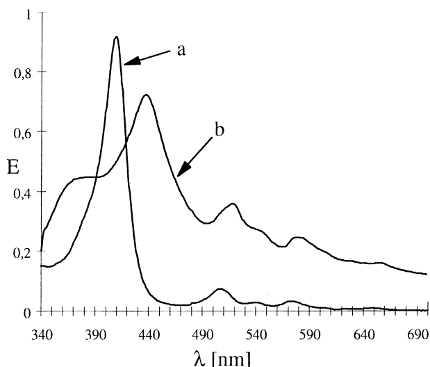
Figure 1. Optical spectra of porphyrin 13 in \text{CHCl}_3 (a) and PBS-solution (b).
