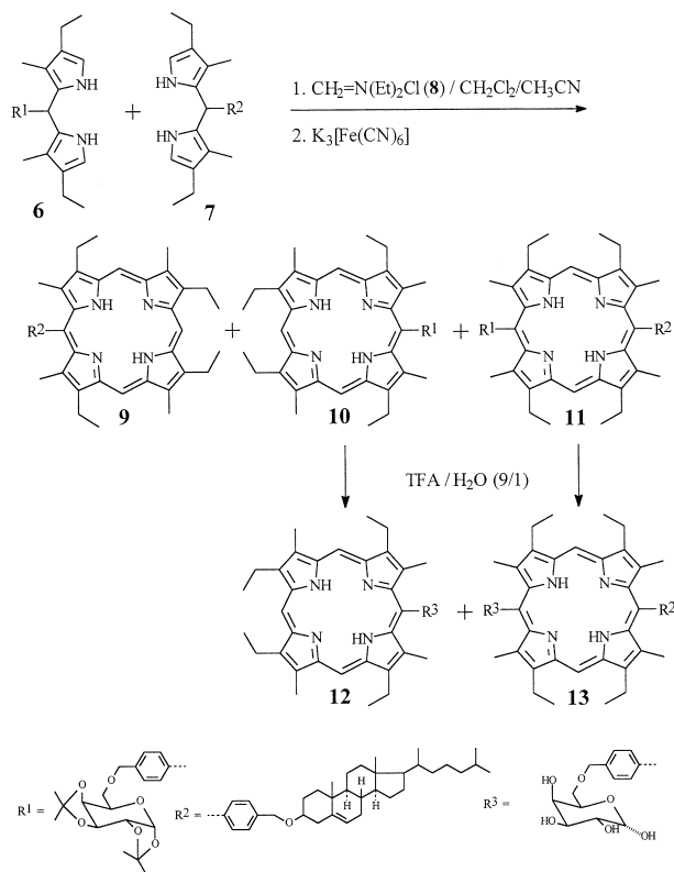
Scheme 2. Synthesis of porphyrins.
