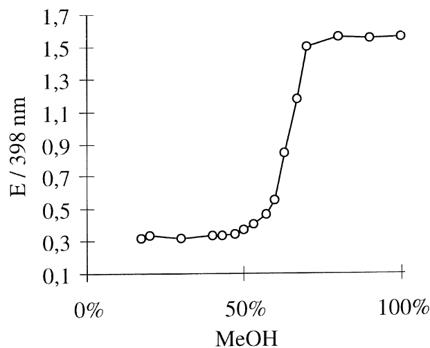
Figure 2. Aggregation curve of 12 in methanol/water mixtures. Absorbance was detected at 398 nm and corrected for density and compression changes.
